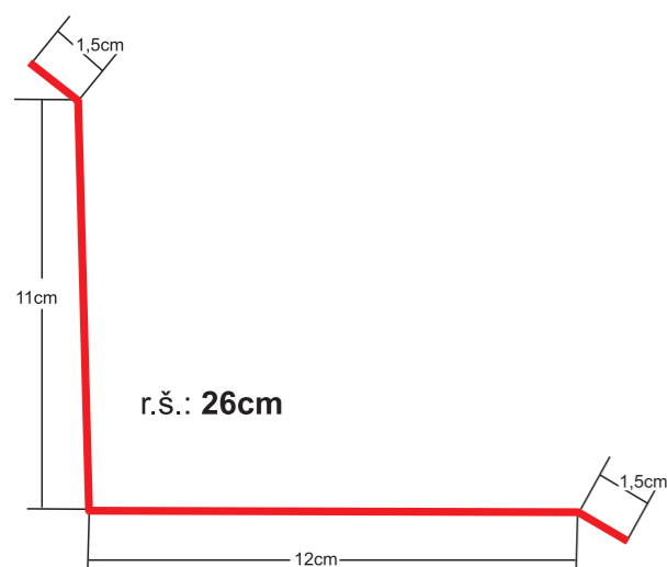
Lemovanie muriva vrchné Upper masonry edging
